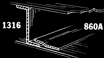
1316 860A DOUBLE WALL PANEL CONSTRUCTION
