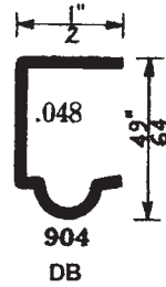
METAL TRIM FOR VISION PANEL
