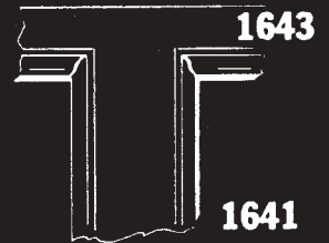
MULLION CASING IN COMBINATION WITH NO. 1643
