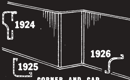
1924 1925 1926 CORNER AND CAP TRIMS FOR PARTITION
